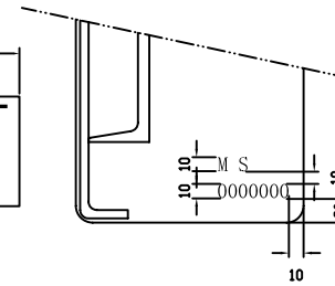
LEFT CORNER FITTING STAMPING OF MANUFACTURE'S SERIAL NO.
